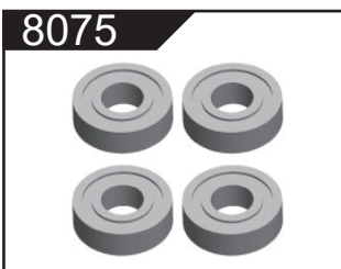
8075 Kugellager 8x12x3.5 (4)
